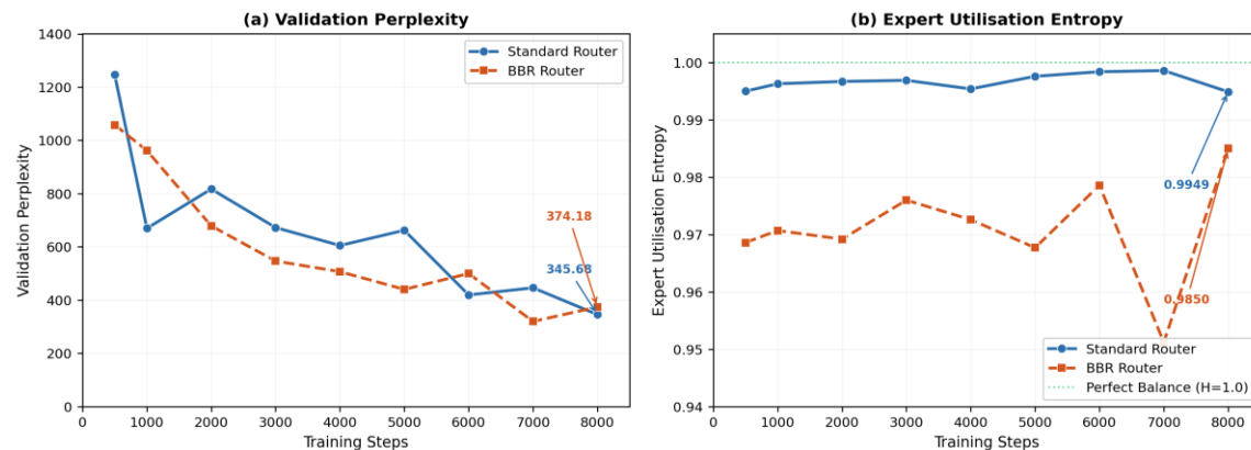
Fig 2. Evolution of Validation Perplexity and Expert utilization entropy
