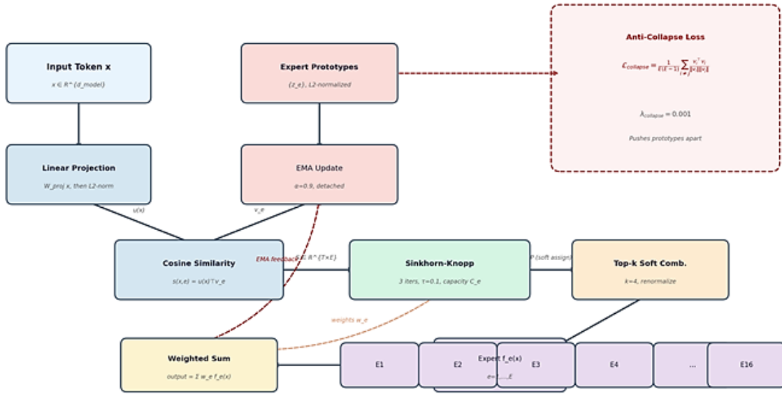
Fig 1. Architecture of the BBR Routing Block
