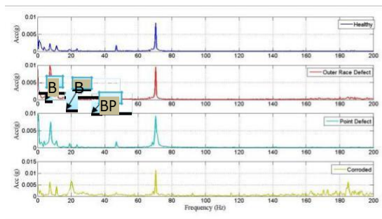
Fig.8. Frequency spectrum for bearings that rotate at 287 rpm
